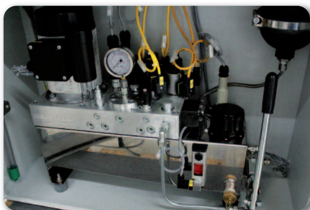
Hydraulic powerpack
